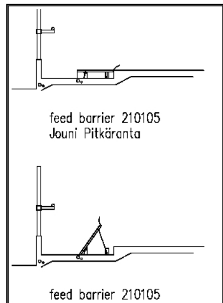
Figure 1. An automated feed barrier with a design similar to the spoilers on the wing of a jet aircraft.
